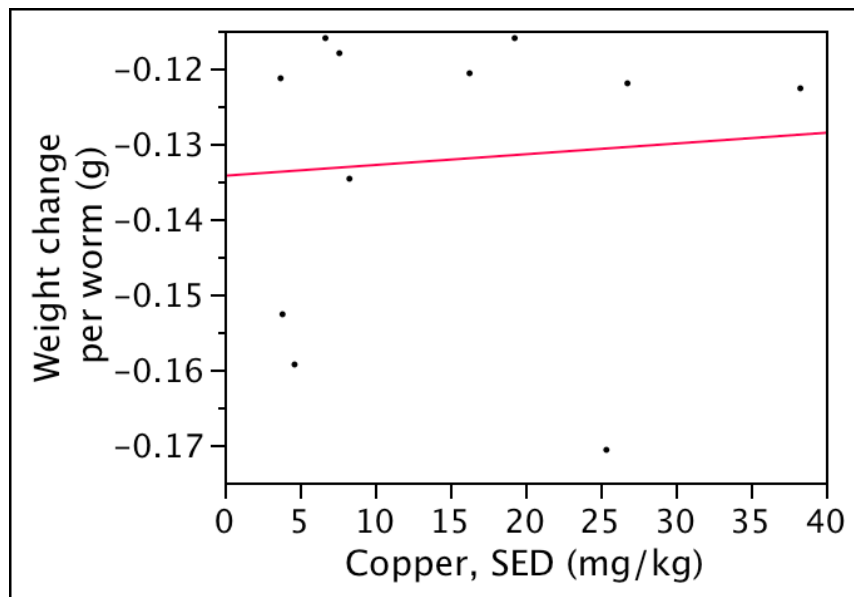
Figure E-1.3-20 Bivariate plot of worm growth versus copper (COPEC). Weight change per worm (g) = -0.134 + 0.000143 \times \text{copper, SED} ; r^2 = 0.00716 ; n = 11 ; p = 0.805 .
