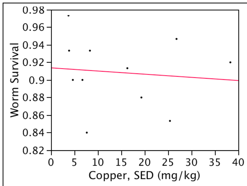
Figure E-1.3-19 Bivariate plot of worm survival versus copper (COPEC). Worm survival = 0.914 - 0.000362 \times \text{copper, SED} ; r^2 = 0.0111 ; n = 11 ; p = 0.758 .
