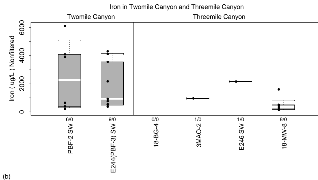
Figure D-2.1-5 Box plots showing the spatial distribution of iron ( \mu\text{g/L} ) at surface water and alluvial groundwater locations in nonfiltered samples (a) in Pajarito Canyon and (b) in Twomile and in Threemile Canyon
