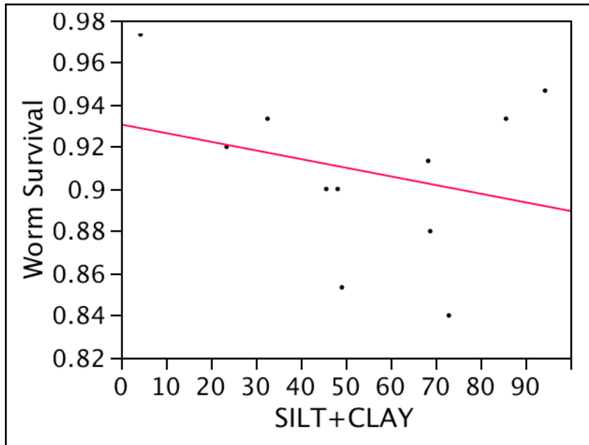
Figure E-1.3-11 Bivariate plot of worm survival versus silt+clay (potential confounding factor). Worm survival = 0.931 - 0.000411 * silt+clay ; r^2 = 0.079 ; n = 11 ; p = 0.402 .
