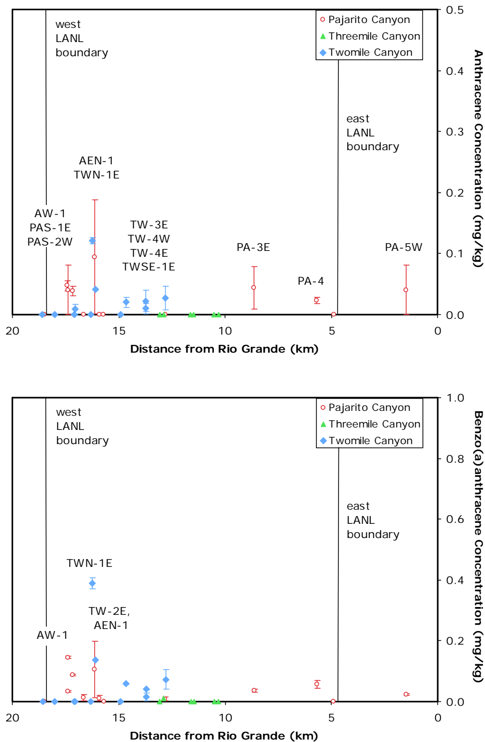
Figure 7.1-3 Estimated average concentrations of select PAHs in fine facies sediment in the Pajarito watershed. Error bars indicate upper and lower bounds based on replacing nondetect values with either the detection limit or zero, and a value of zero is shown where there are no detected results.
