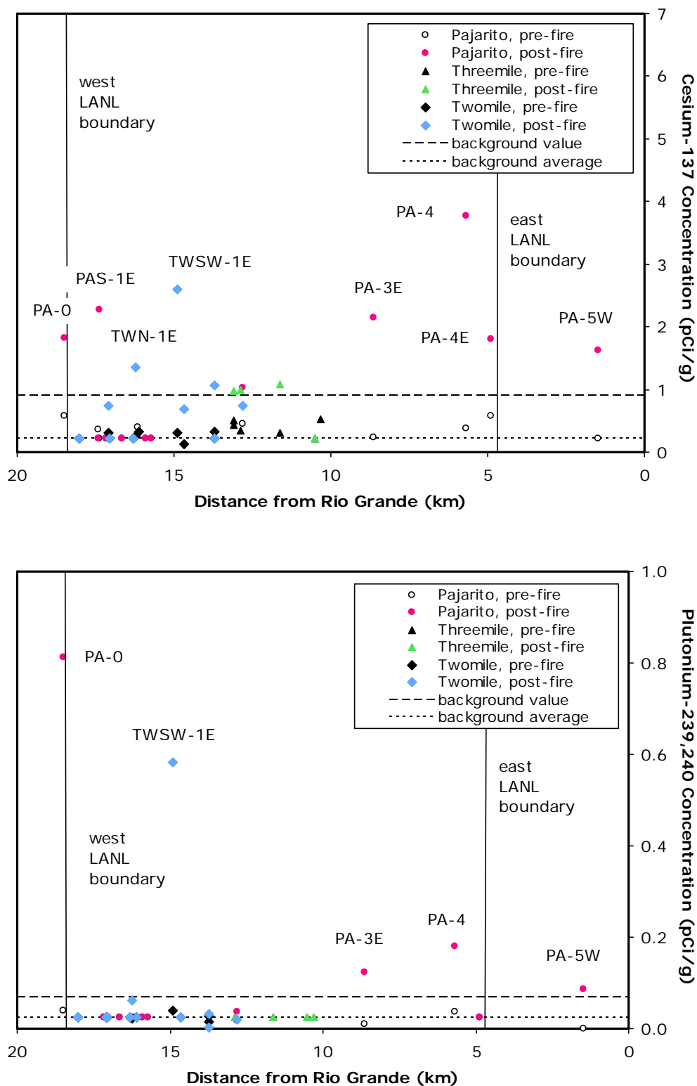
Figure 7.1-8 Estimated average concentrations of cesium-137 and plutonium-239,240 in fine facies sediment in the Pajarito watershed; value shown as the average background concentration in reaches where these radionuclides are not COPCs.
