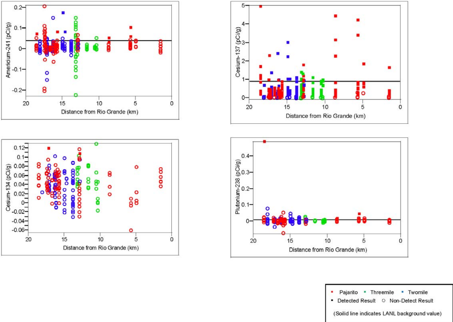
Figure D-1.1-3 Plots of sample results versus distance from the Rio Grande for all radionuclide COPCs identified in sediment in the Pajarito watershed
