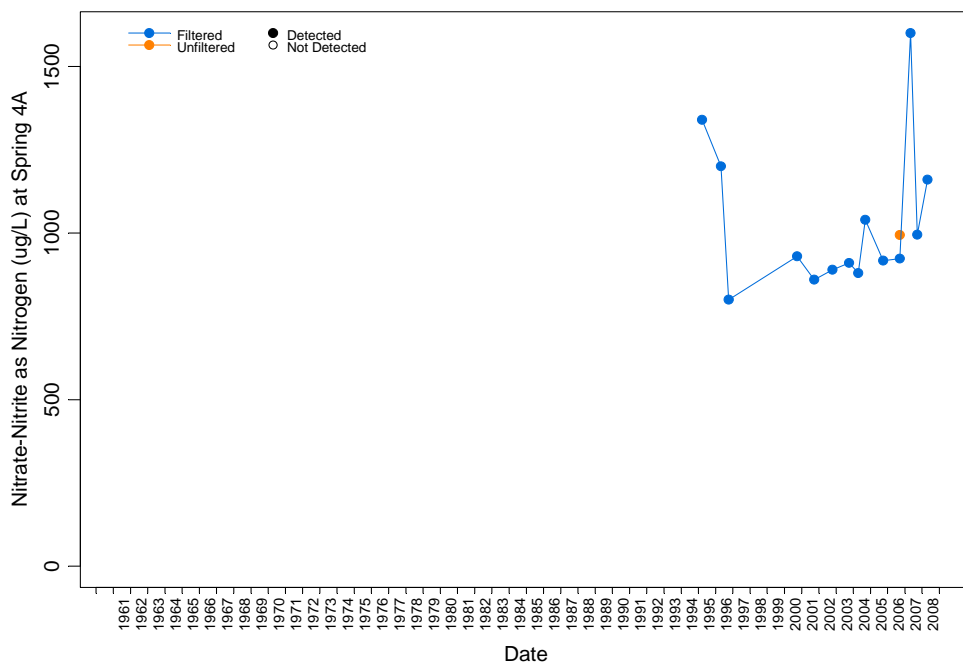
Figure D-2.2-162 Concentrations over time at Spring 4A for nitrate-nitrite as nitrogen
