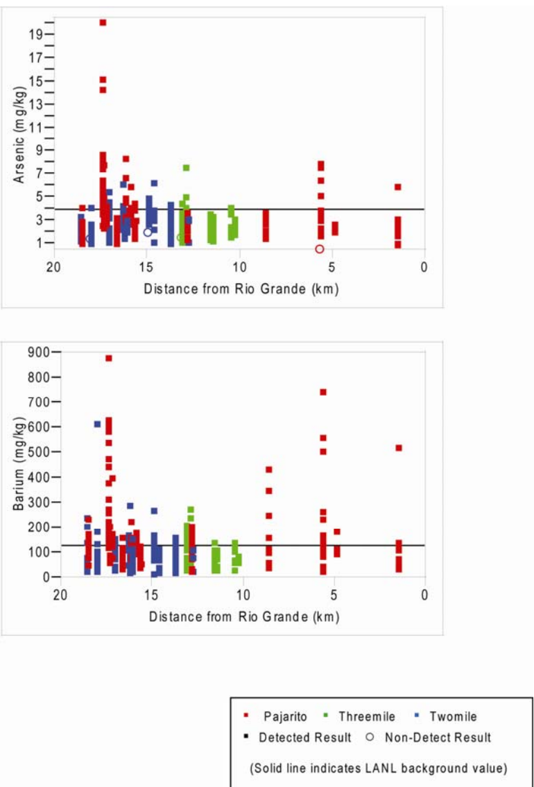
Figure D-1.1-1 Plots of sample results versus distance from the Rio Grande for all inorganic COPCs identified in sediment in the Pajarito watershed
