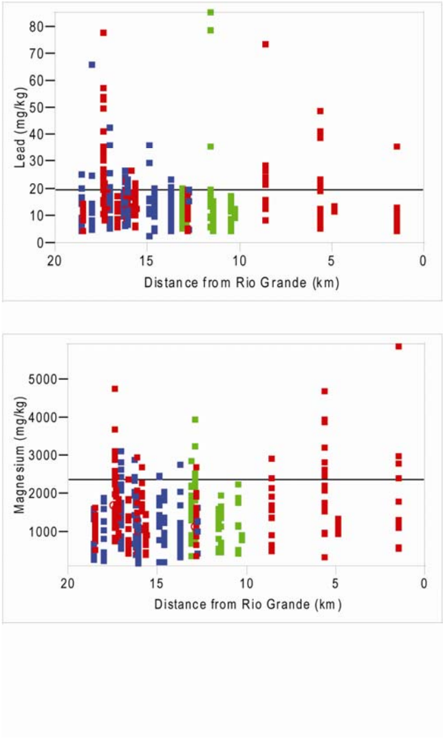
Figure D-1.1-1 (continued)
