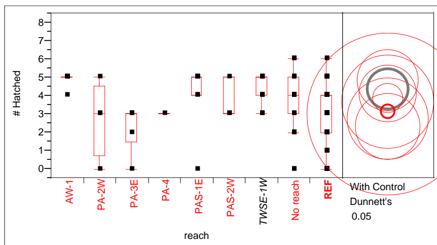
Figure E-1.2-30 Box plots of number hatched for all species by reach
