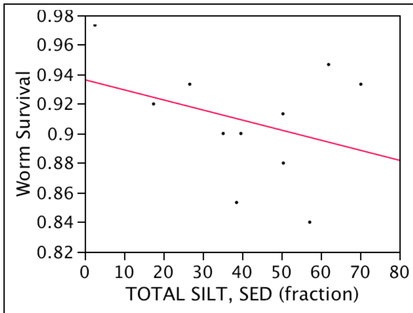
Figure E-1.3-7 Bivariate plot of worm survival versus total silt (potential confounding factor). Worm survival = 0.936 - 0.000681 \times \text{total silt, SED} ; r^2 = 0.118 ; n = 11 ; p = 0.301 .
