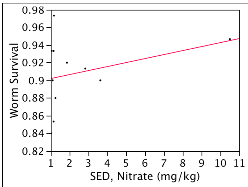
Figure E-1.3-1 Bivariate plot of worm survival versus nitrate (potential confounding factor). Worm survival = 0.897 + 0.00453 \times \text{SED, nitrate} ; r^2 = 0.103 ; n = 11 ; p = 0.336 .
