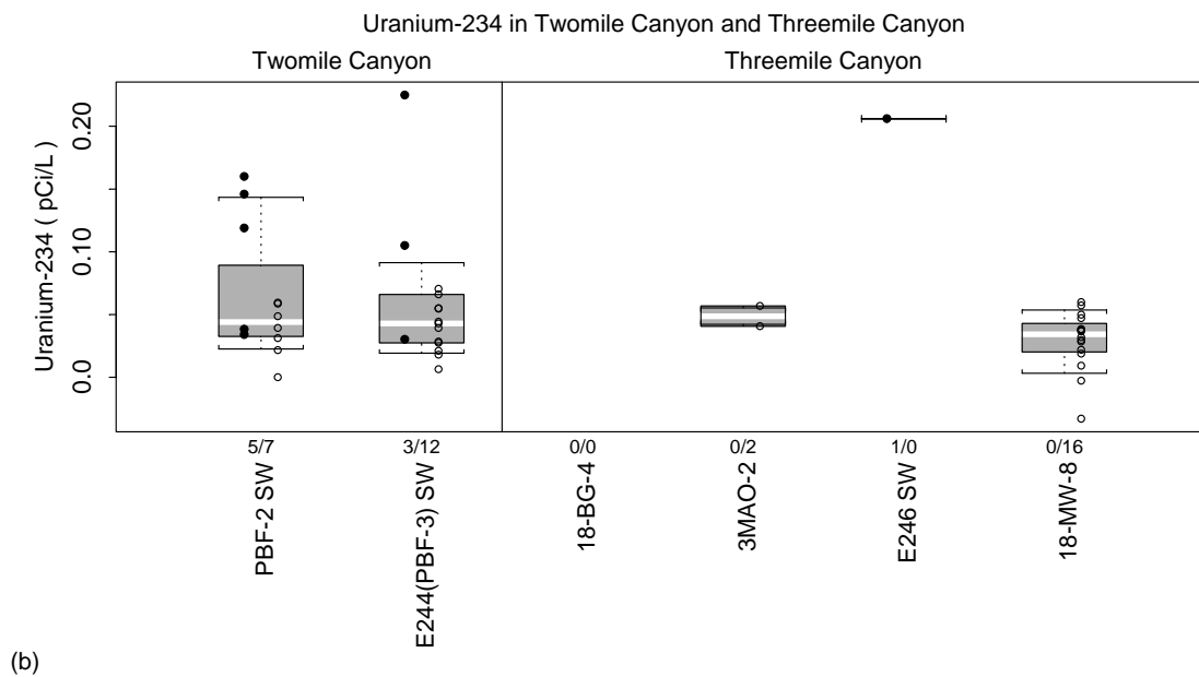
Figure D-2.1-10 Box plots showing the spatial distribution of uranium-234 (pCi /L) at surface water and alluvial groundwater locations in both filtered and nonfiltered samples (a) in Pajarito Canyon and (b) in Twomile and in Threemile Canyon
